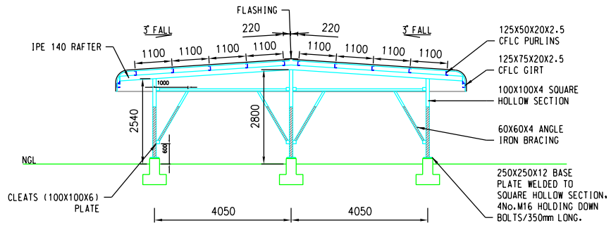
VERTICAL BRACING TYPE 2 SCALE 1:10
